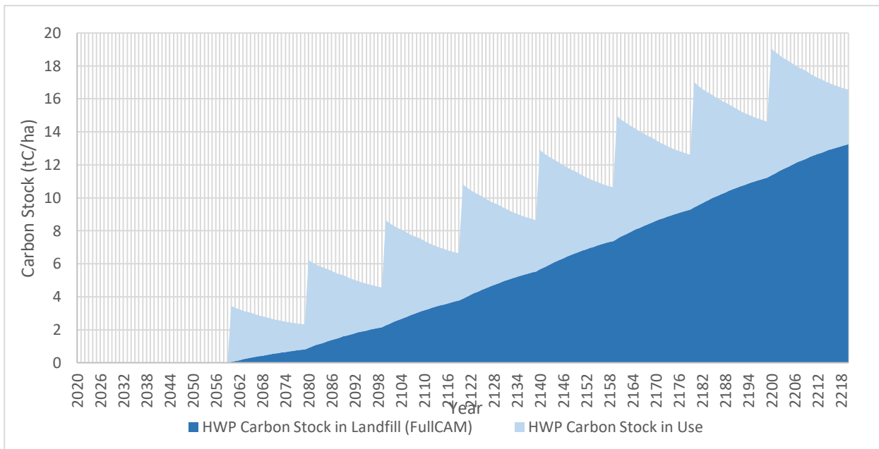
Figure 8.7. Harvested wood product carbon stock in use (light blue area) and deposited in landfill (dark blue area) over the Scenario 2 study period for for coastal dry eucalypt forest in the North East NSW Hub region.
